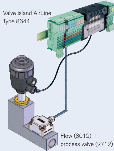
On/Off control loop
