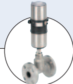
Type 8802-GD TopControl System
